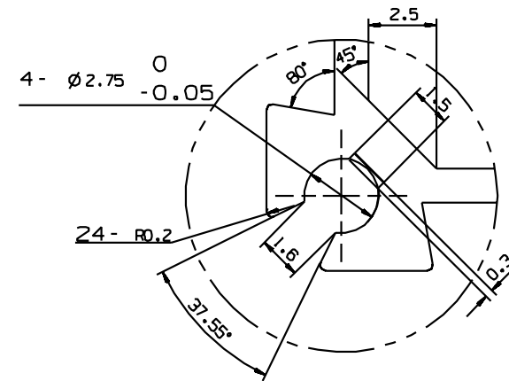
DETAIL A SCALE 6:1
