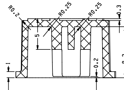
SECTION J - J
