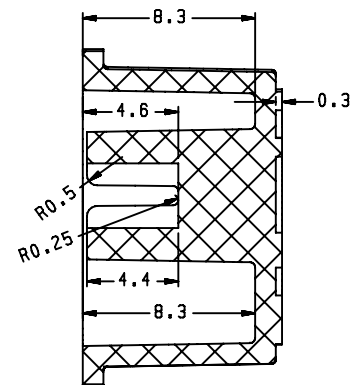
SECTION K - K
